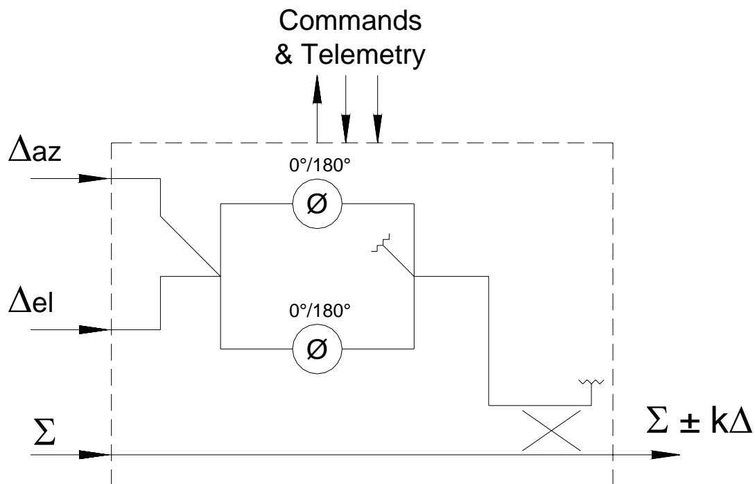
Figure 5. Autotrack modulator configuration incorporating dual 180^\circ phase shifters between magic tees.
