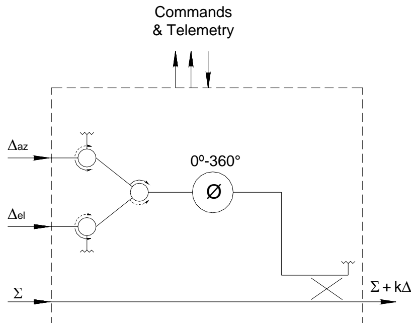
Figure 9. The phase shifter based autotrack modulator incorporates a high-isolation RF switch and a high-resolution ferrite phase shifter. The high-resolution phase shifter enables electronic phase trimming within the autotrack.
