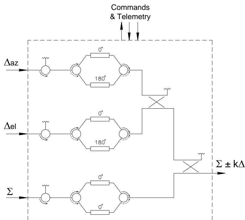
Figure 7. Schematic of a switched-line autotrack modulator. Switched-line modulators with ferrite switches offer the lowest insertion loss of any ATM approach.
