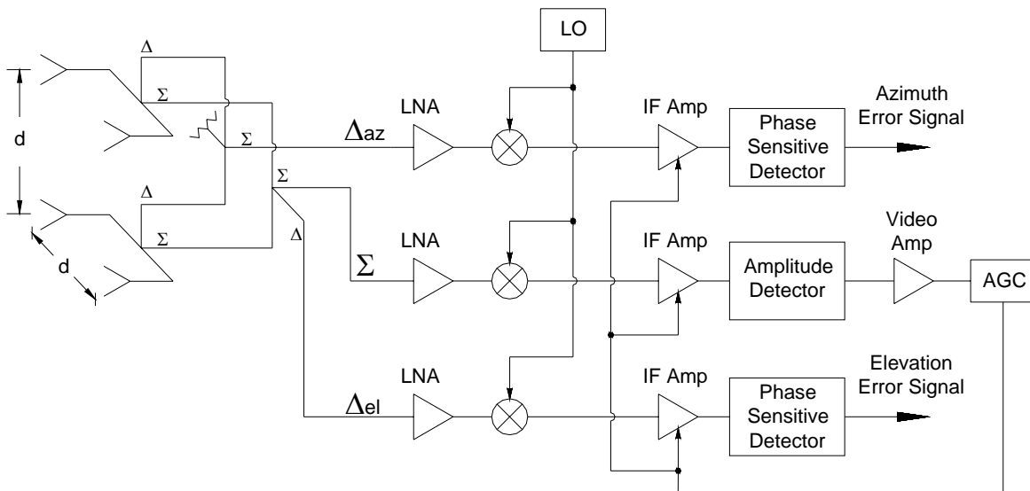
Figure 1. A three-channel monopulse receiver system
