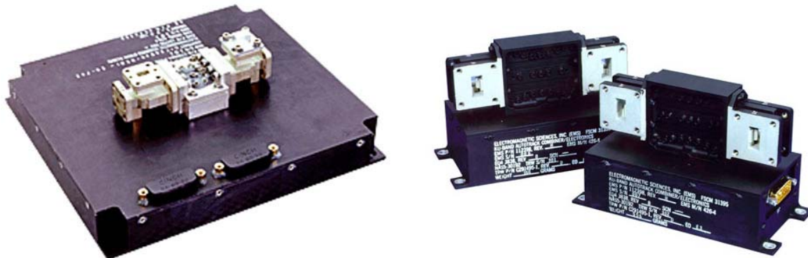
Figure 6. Phase shifter/tee autotrack modulators built for the ACTS (left) and TDRS A-G (right) spacecraft. The ACTS unit operates at K a -band and the TDRS unit at K u -band.
