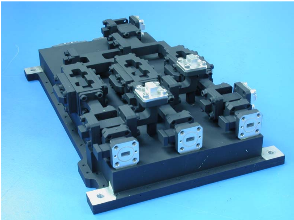
Figure 8. A K_a -band switched line autotrack modulator. This unit includes sampling couplers on all of the input ports for use in alignment.
