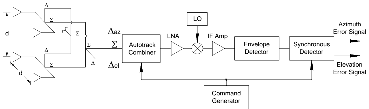
Figure 2. The autotrack combiner allows monopulse tracking to be accomplished with a single-channel receiver.
