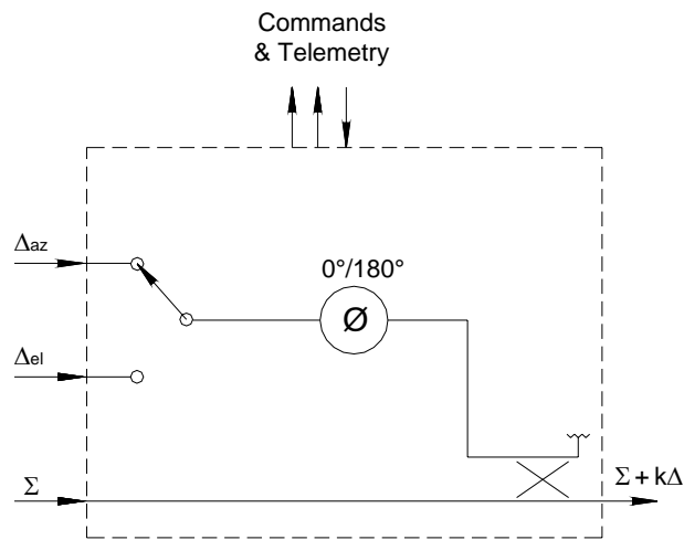
Figure 3. Generic autotrack combiner schematic
